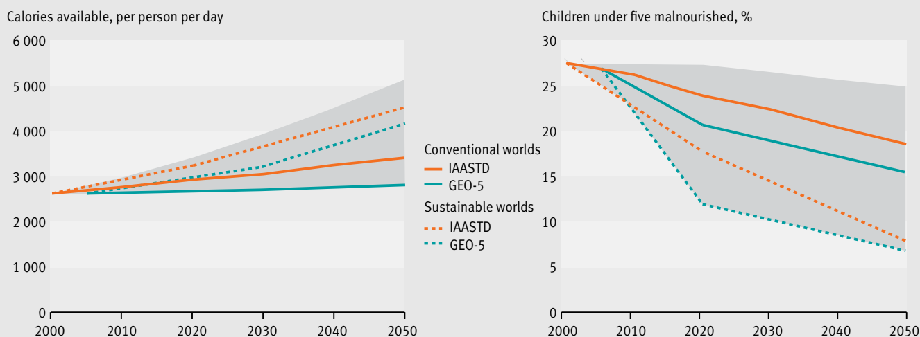
Figure 16.8 Food consumption and child undernourishment under different scenarios
