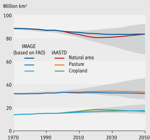
Figure 16.9 Trends in land use, 1970–2050
